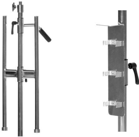
Pump holder for side-by-side mounting, handle and power socket holder. Removable and height adjustable.
