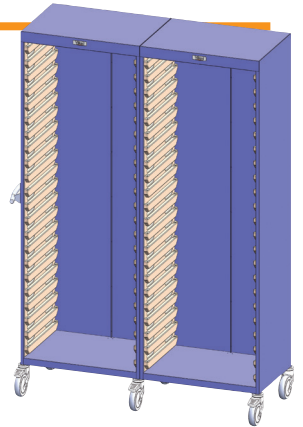
Ref. 1007.06 128 x 46 x 195 HT cm 2 x 22 levels
