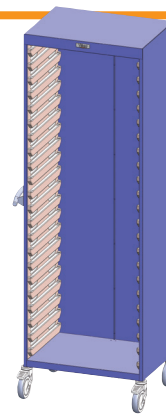
Ref. 1007.01 64 x 46 x 195 HT cm 22 levels
