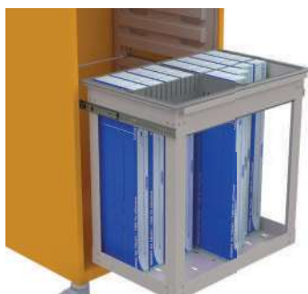
Telescopic support for packed probes
